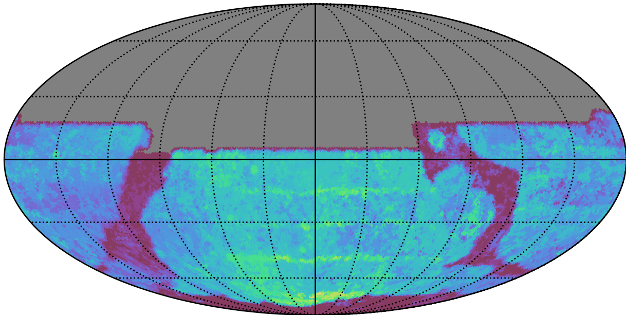
ddf_acor_sf25_lsf30_lsr50_v3.4_10yrs All sky y band: Median Season Length
