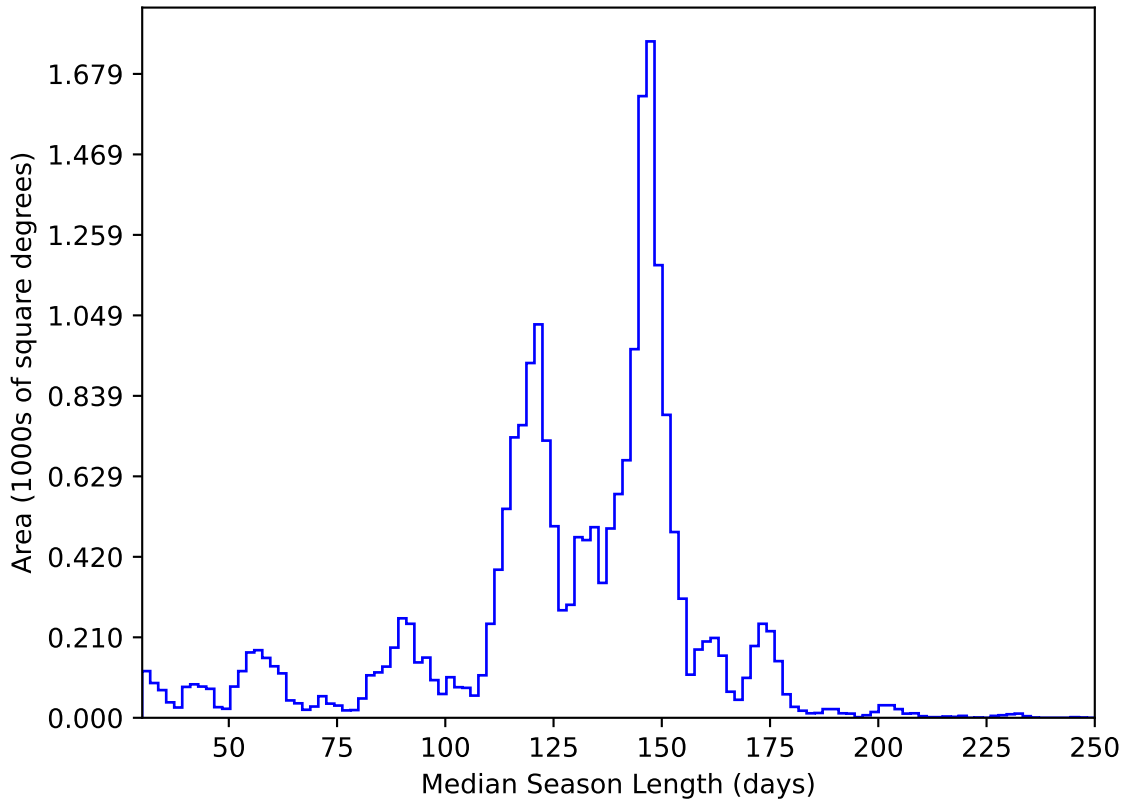
ddf_acor_sf25_lsf30_lsr50_v3.4_10yrs All sky y band: Median Season Length
