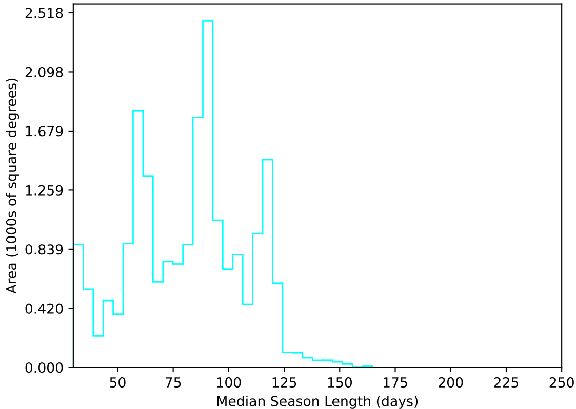
ddf_acor_sf25_lsf30_lsr50_v3.4_10yrs All sky u band: Median Season Length
