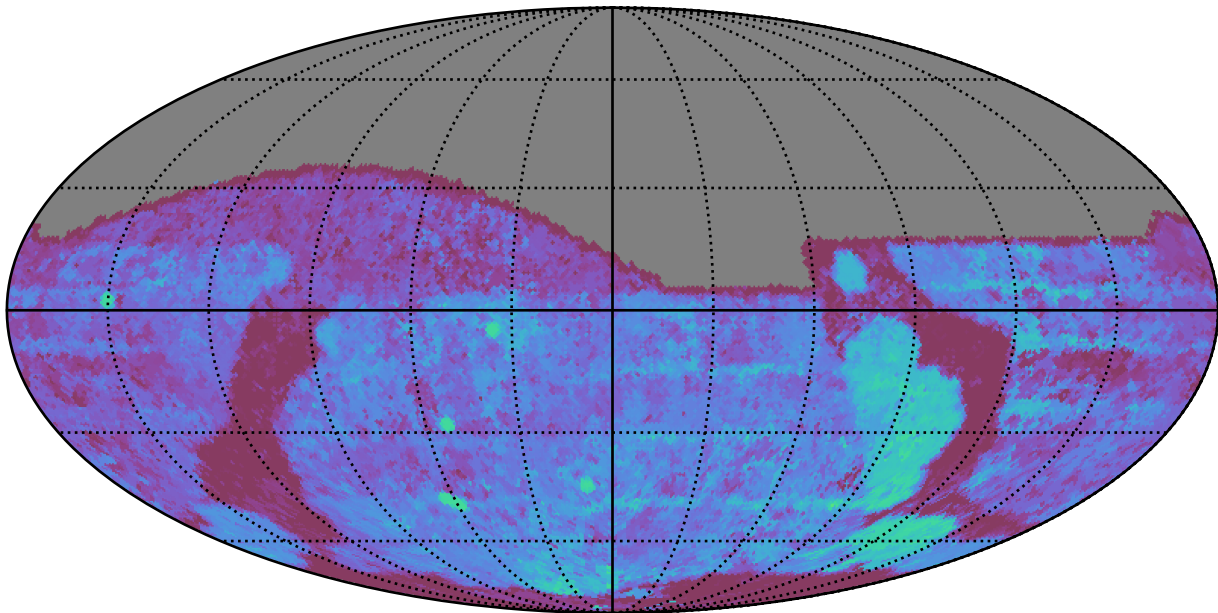
ddf_acor_sf25_lsf30_lsr50_v3.4_10yrs All sky g band: Median Season Length
