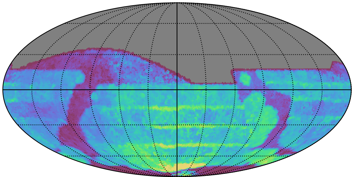
ddf_acor_sf25_lsf30_lsr50_v3.4_10yrs All sky all bands: Median Season Length
