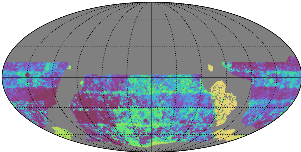
ddf_acor_sf25_lsf30_lsr50_v3.4_10yrs WFD y band: Median Inter-Night Gap
