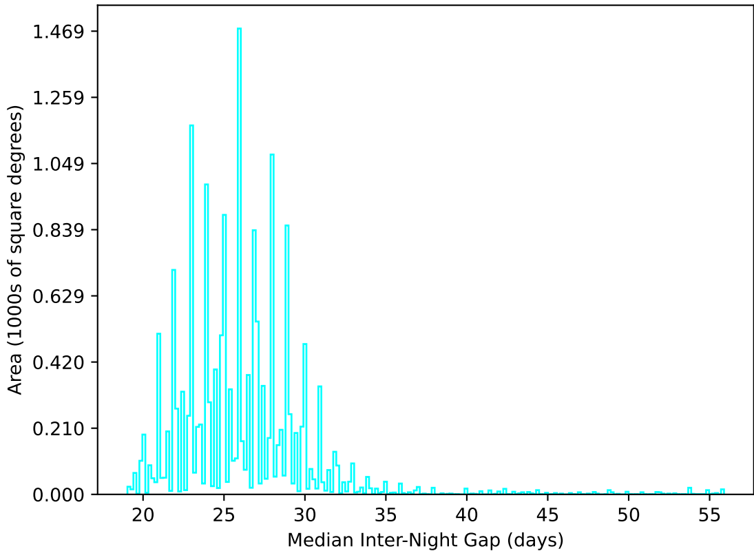
ddf_acor_sf25_lsf30_lsr50_v3.4_10yrs WFD u band: Median Inter-Night Gap
