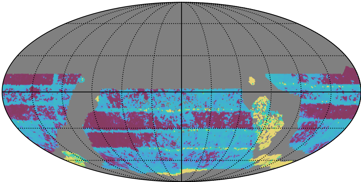
ddf_acor_sf25_lsf30_lsr50_v3.4_10yrs WFD all bands: Median Inter-Night Gap
