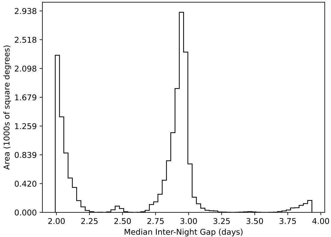
ddf_acor_sf25_lsf30_lsr50_v3.4_10yrs WFD all bands: Median Inter-Night Gap
