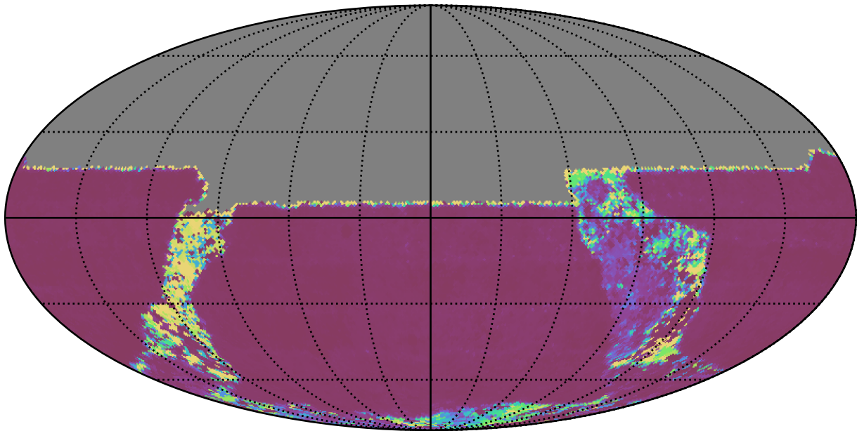
ddf_acor_sf25_lsf30_lsr50_v3.4_10yrs All sky u band: Median Inter-Night Gap
