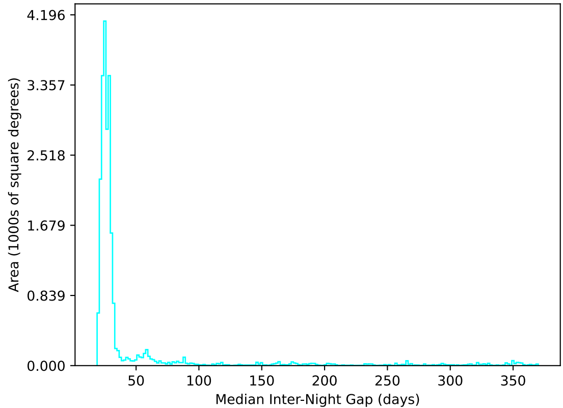
ddf_acor_sf25_lsf30_lsr50_v3.4_10yrs All sky u band: Median Inter-Night Gap
