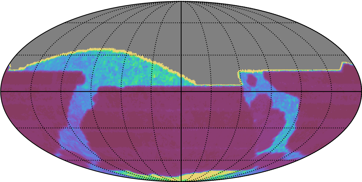
ddf_acor_sf25_lsf30_lsr50_v3.4_10yrs All sky all bands: Median Inter-Night Gap
