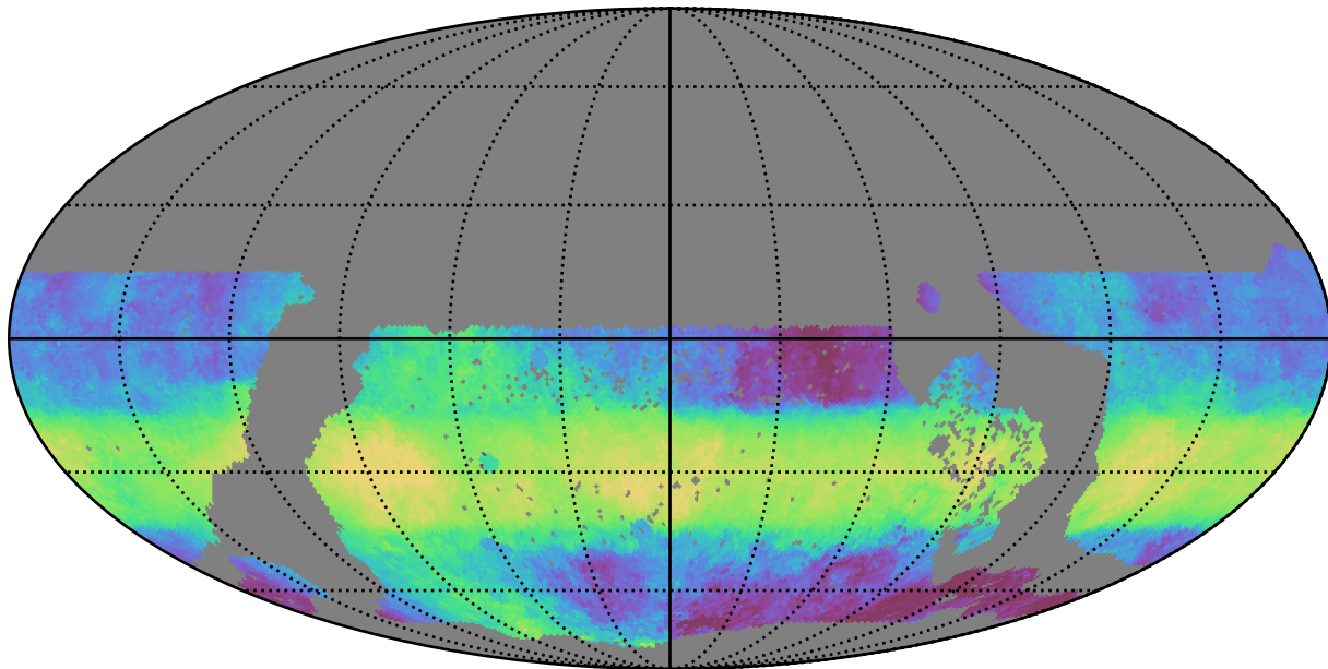
ddf_acor_sf25_lsf30_lsr50_v3.4_10yrs WFD z band: Median HA
