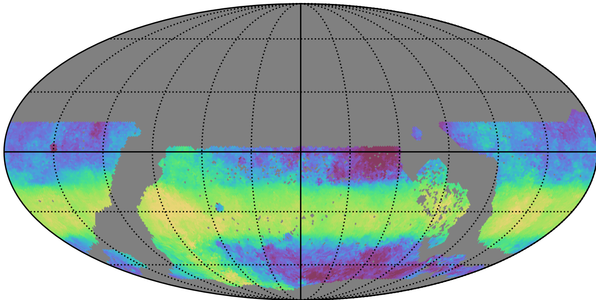
ddf_acor_sf25_lsf30_lsr50_v3.4_10yrs WFD y band: Median HA
