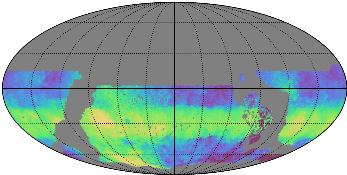
ddf_acor_sf25_lsf30_lsr50_v3.4_10yrs WFD u band: Median HA
