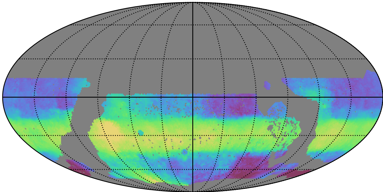
ddf_acor_sf25_lsf30_lsr50_v3.4_10yrs WFD r band: Median HA
