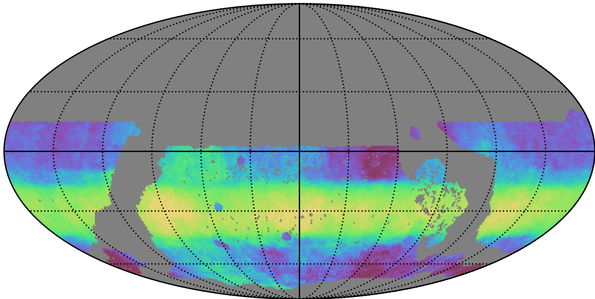
ddf_acor_sf25_lsf30_lsr50_v3.4_10yrs WFD i band: Median HA
