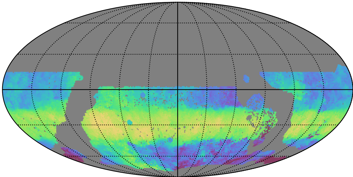
ddf_acor_sf25_lsf30_lsr50_v3.4_10yrs WFD g band: Median HA
