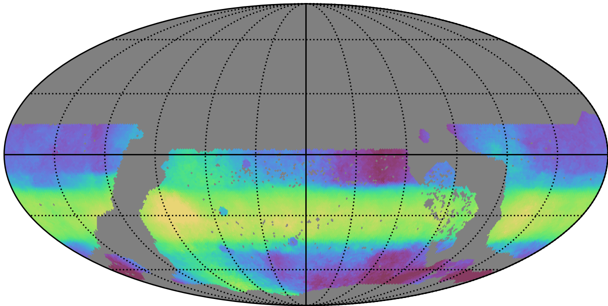
ddf_acor_sf25_lsf30_lsr50_v3.4_10yrs WFD all bands: Median HA
