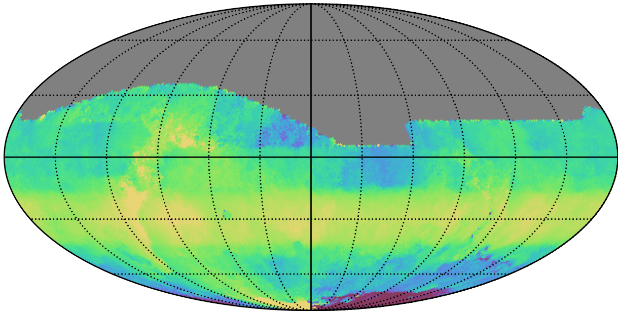
ddf_acor_sf25_lsf30_lsr50_v3.4_10yrs All sky z band: Median HA
