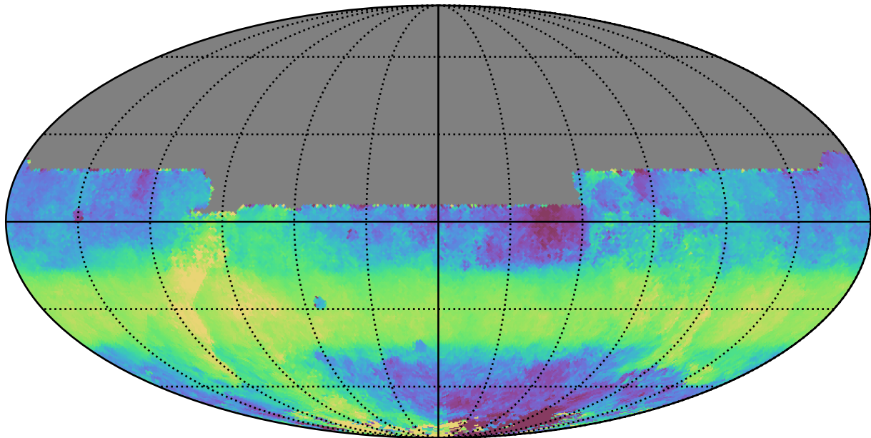
ddf_acor_sf25_lsf30_lsr50_v3.4_10yrs All sky y band: Median HA
