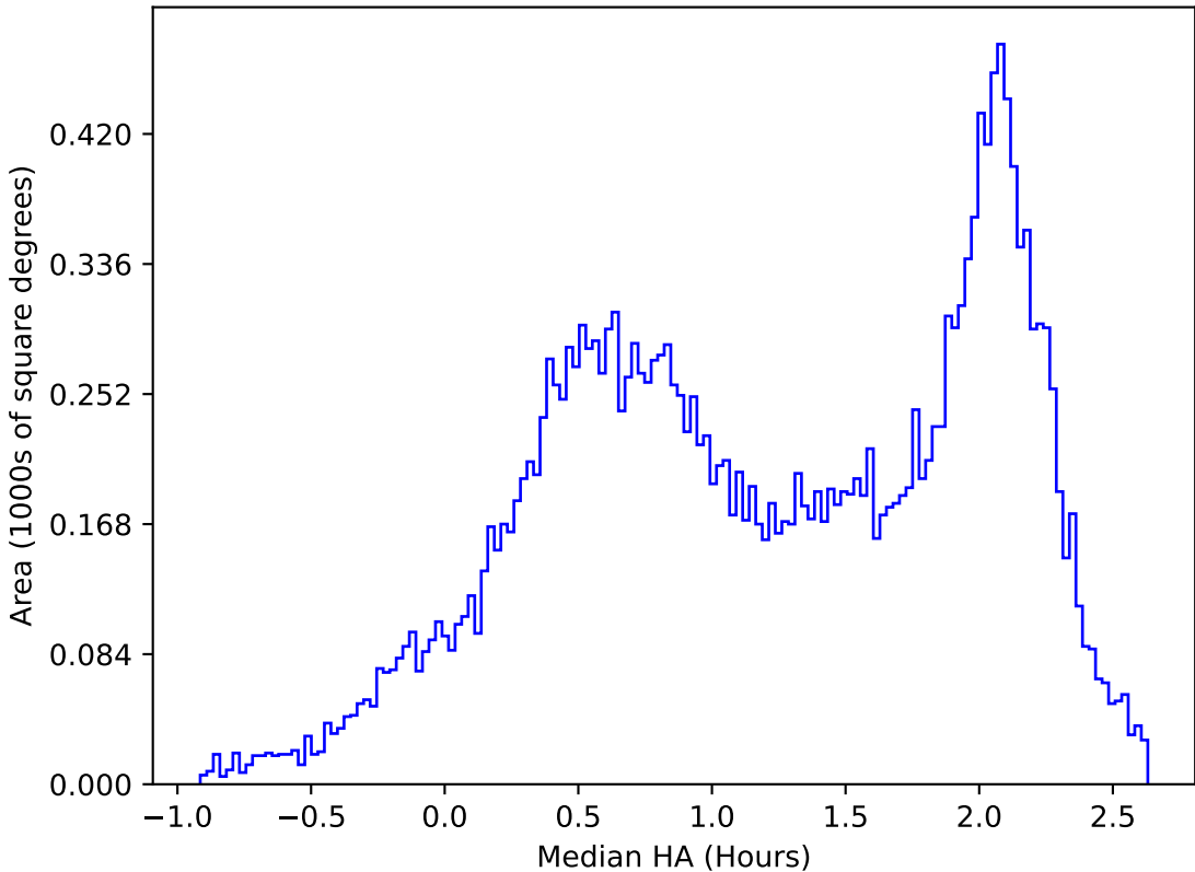
ddf_acor_sf25_lsf30_lsr50_v3.4_10yrs All sky y band: Median HA
