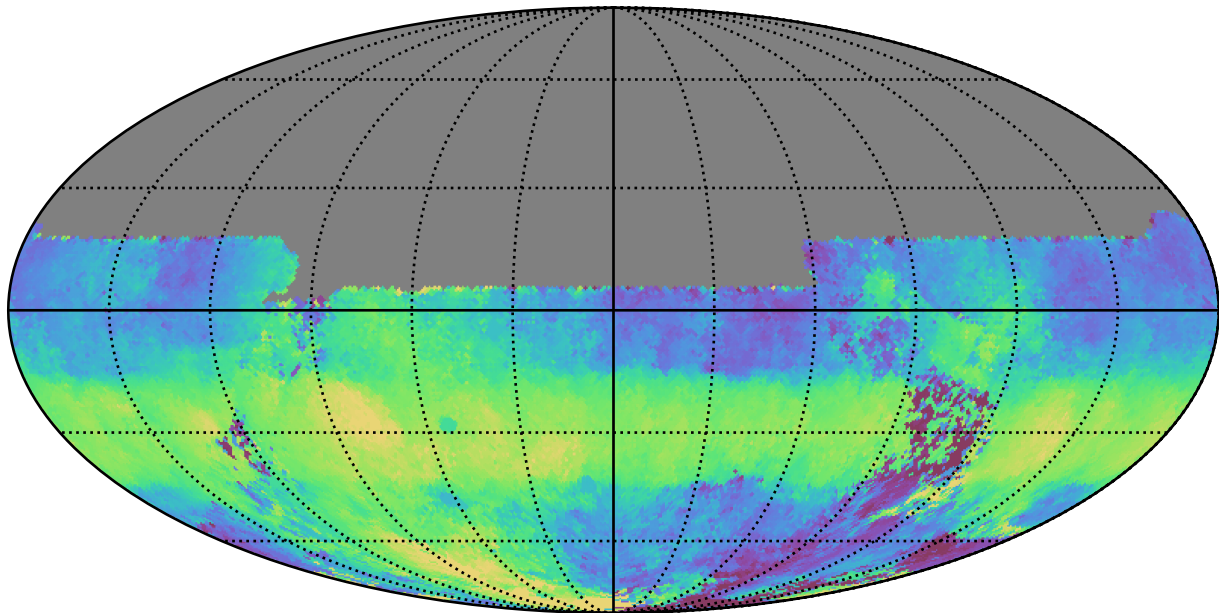
ddf_acor_sf25_lsf30_lsr50_v3.4_10yrs All sky u band: Median HA
