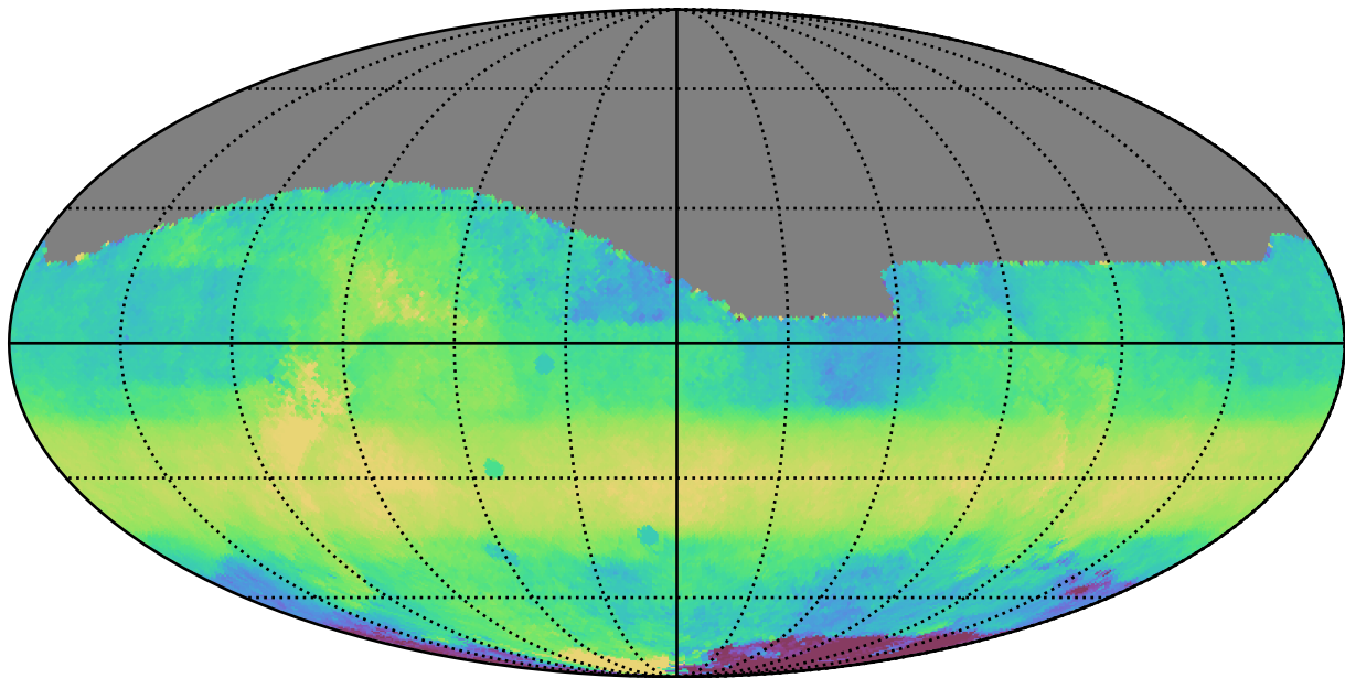
ddf_acor_sf25_lsf30_lsr50_v3.4_10yrs All sky i band: Median HA
