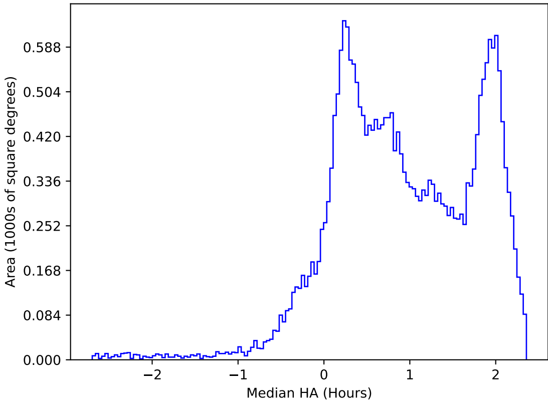
ddf_acor_sf25_lsf30_lsr50_v3.4_10yrs All sky i band: Median HA
