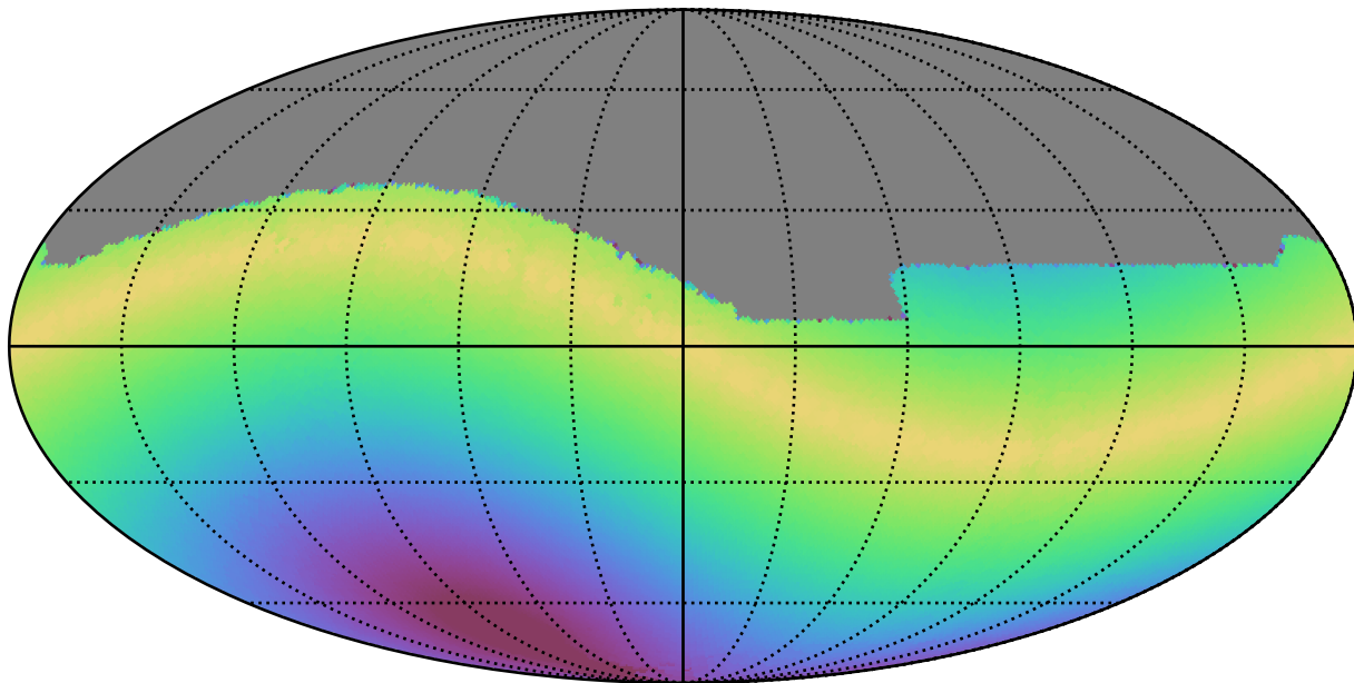
ddf_acor_sf25_lsf30_lsr50_v3.4_10yrs All sky i band: Max solarElong
