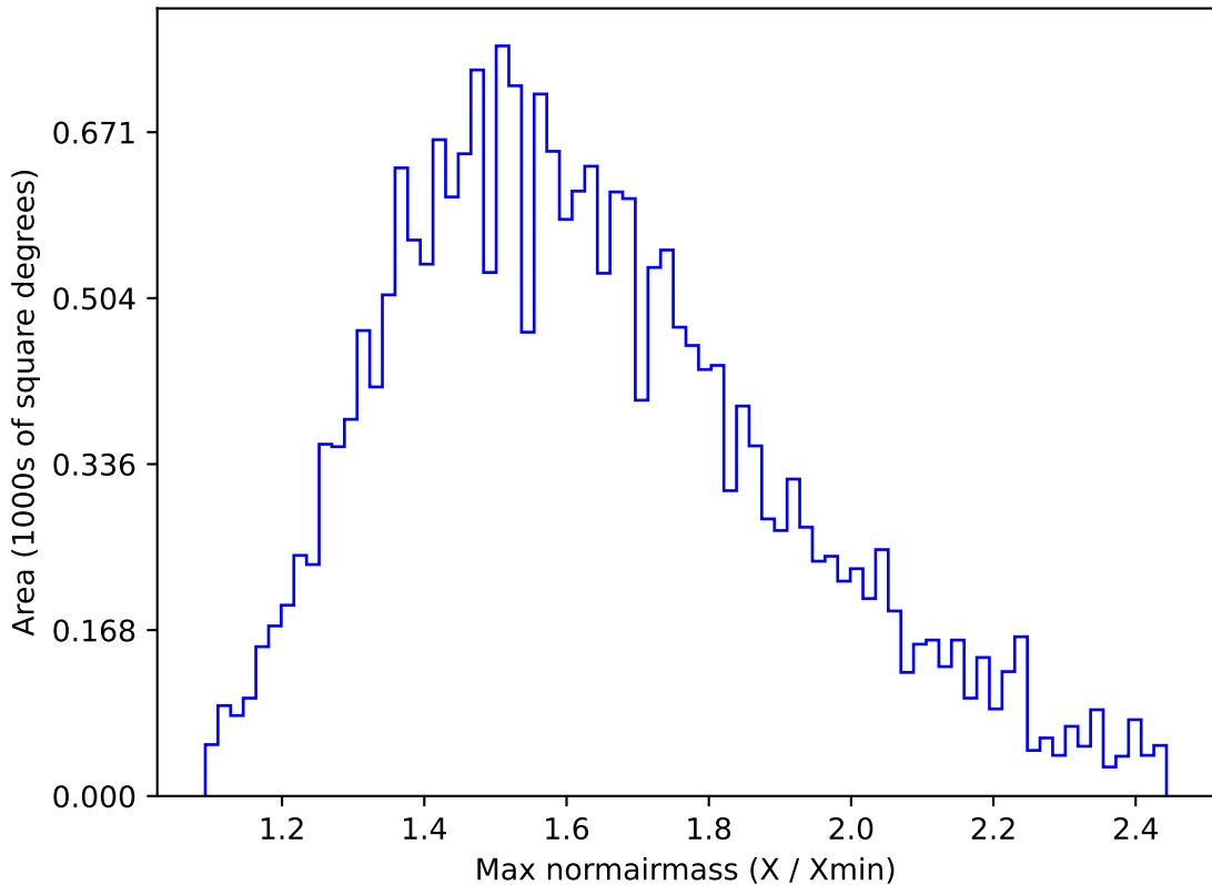
ddf_acor_sf25_lsf30_lsr50_v3.4_10yrs All sky u band: Max normairmass
