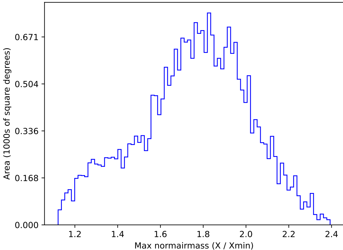
ddf_acor_sf25_lsf30_lsr50_v3.4_10yrs All sky g band: Max normairmass
