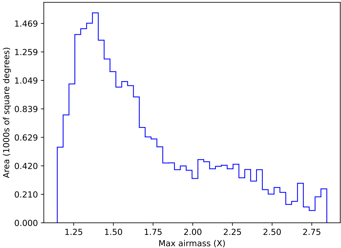
ddf_acor_sf25_lsf30_lsr50_v3.4_10yrs Yr 1 z band: Max airmass
