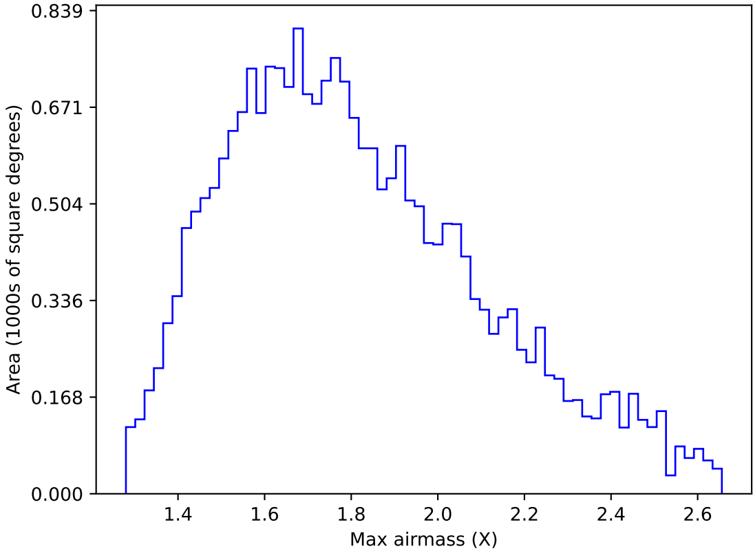
ddf_acor_sf25_lsf30_lsr50_v3.4_10yrs All sky u band: Max airmass
