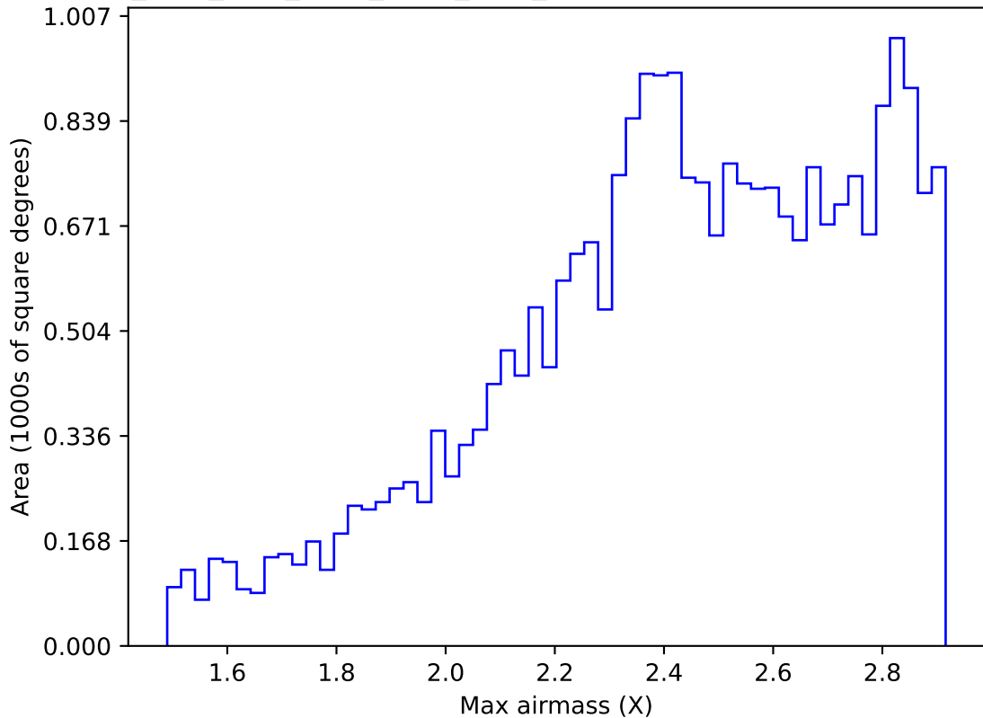
ddf_acor_sf25_lsf30_lsr50_v3.4_10yrs All sky i band: Max airmass
