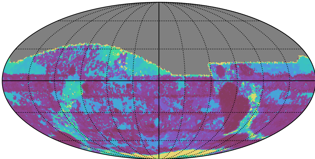
ddf_acor_sf25_lsf30_lsr50_v3.4_10yrs All sky g band: Max Inter-Night Gap
