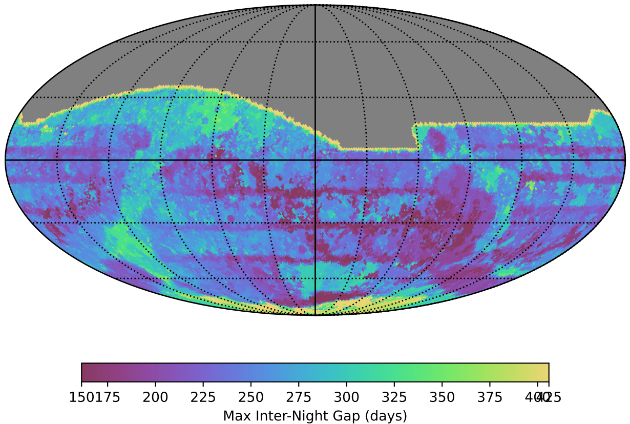
ddf_acor_sf25_lsf30_lsr50_v3.4_10yrs All sky all bands: Max Inter-Night Gap
