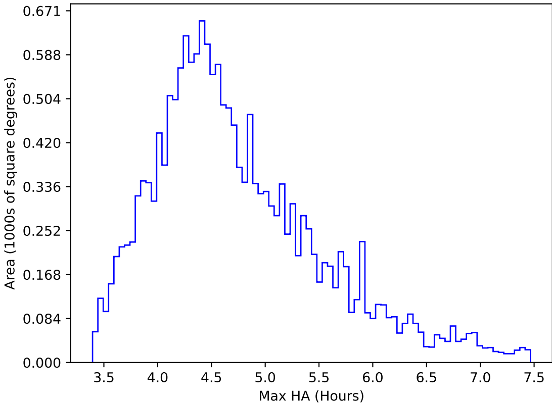
ddf_acor_sf25_lsf30_lsr50_v3.4_10yrs WFD y band: Max HA
