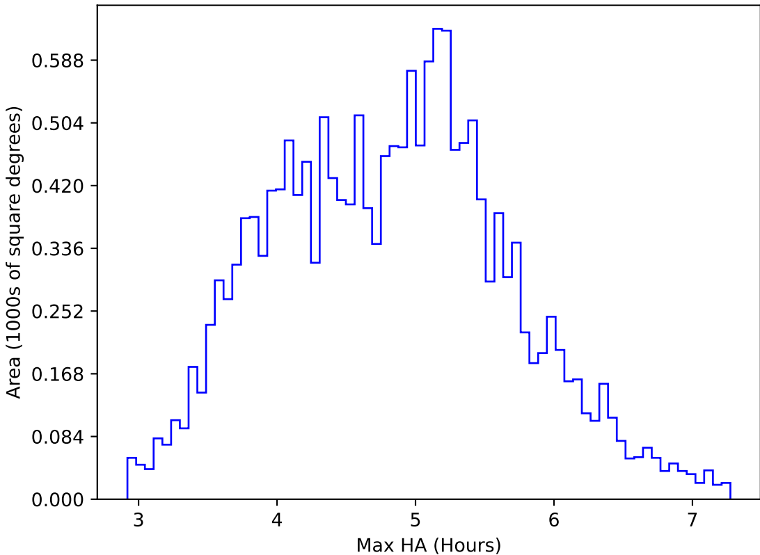
ddf_acor_sf25_lsf30_lsr50_v3.4_10yrs WFD i band: Max HA
