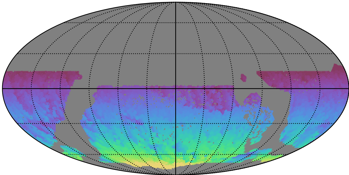
ddf_acor_sf25_lsf30_lsr50_v3.4_10yrs WFD all bands: Max HA
