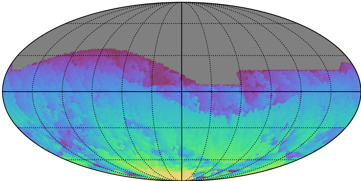
ddf_acor_sf25_lsf30_lsr50_v3.4_10yrs All sky z band: Max HA
