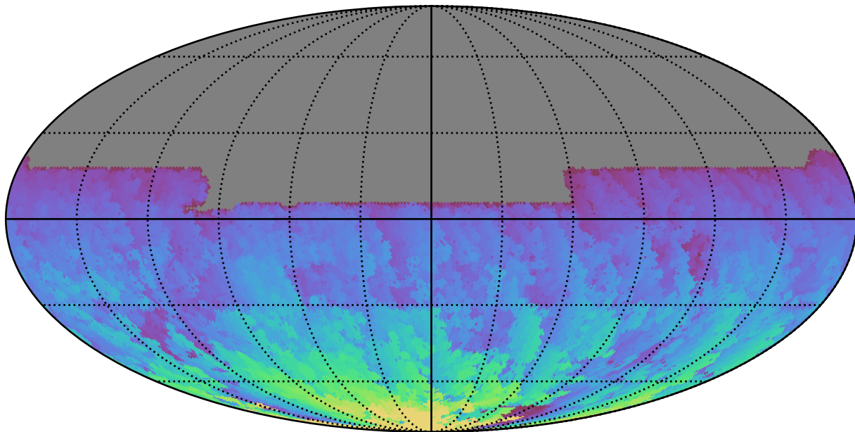
ddf_acor_sf25_lsf30_lsr50_v3.4_10yrs All sky y band: Max HA
