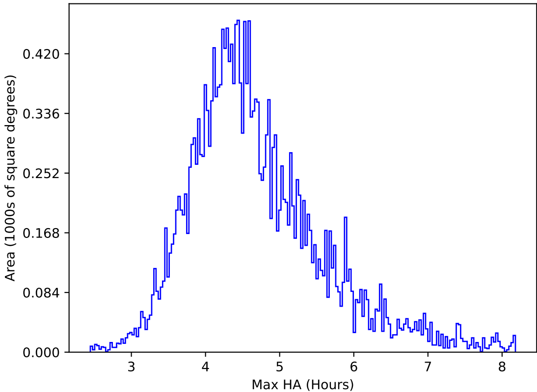
ddf_acor_sf25_lsf30_lsr50_v3.4_10yrs All sky y band: Max HA
