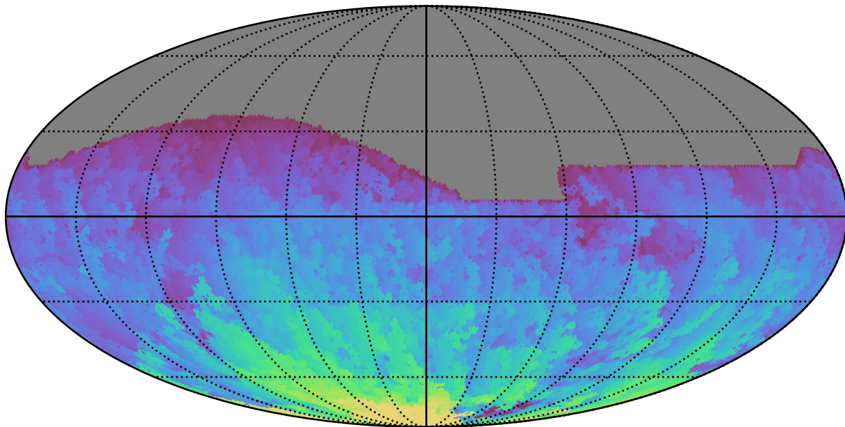
ddf_acor_sf25_lsf30_lsr50_v3.4_10yrs All sky r band: Max HA
