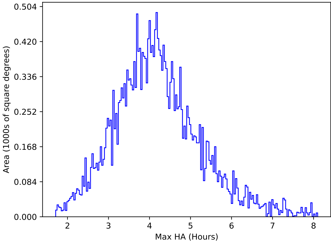
ddf_acor_sf25_lsf30_lsr50_v3.4_10yrs All sky r band: Max HA
