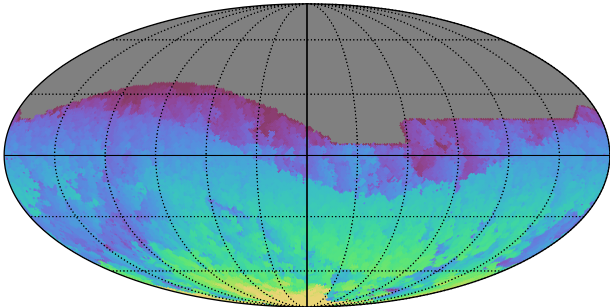
ddf_acor_sf25_lsf30_lsr50_v3.4_10yrs All sky i band: Max HA
