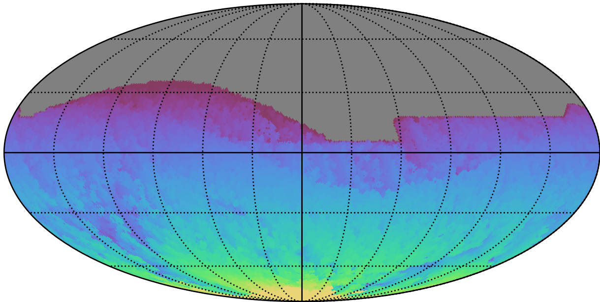
ddf_acor_sf25_lsf30_lsr50_v3.4_10yrs All sky all bands: Max HA
