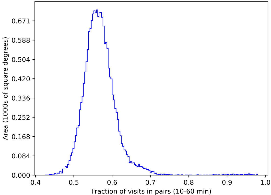
ddf_acor_sf25_lsf30_lsr50_v3.4_10yrs gri WFD: Fraction of visits in pairs (10-60 min)
