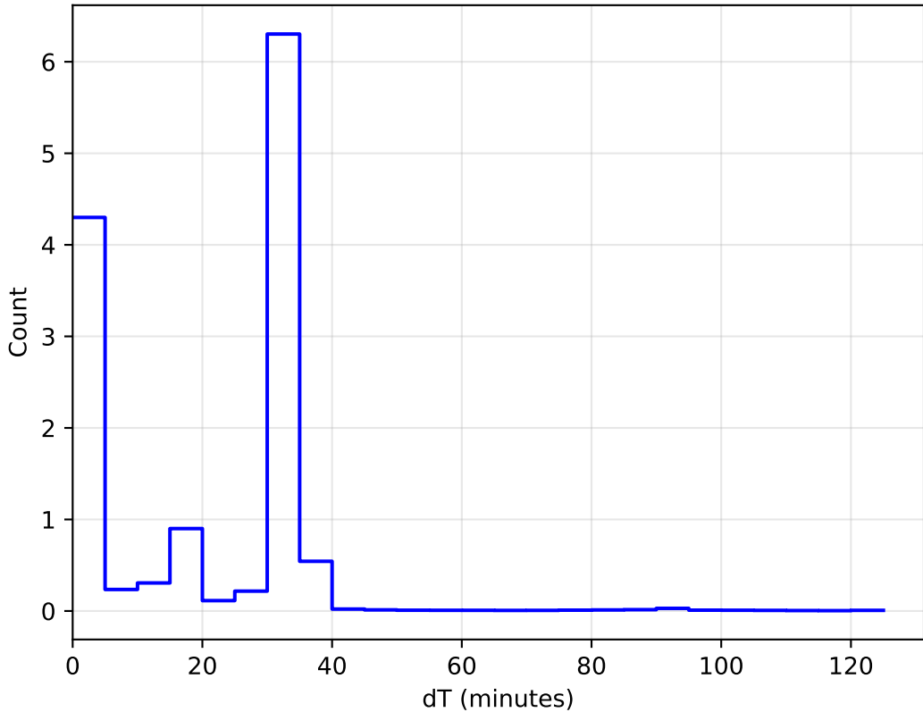
ddf_acor_sf25_lsf30_lsr50_v3.4_10yrs All sky: DeltaT Histogram
