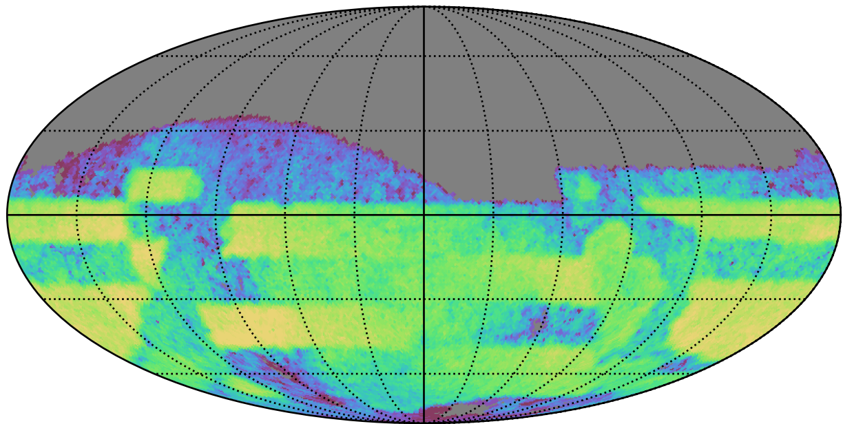
ddf_acor_sf25_lsf30_lsr50_v3.4_10yrs Yr 3-4 i band: CoaddM5
