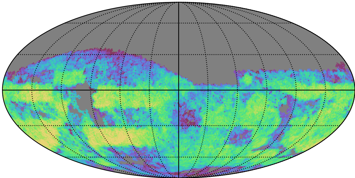
ddf_acor_sf25_lsf30_lsr50_v3.4_10yrs Yr 3-4 g band: CoaddM5
