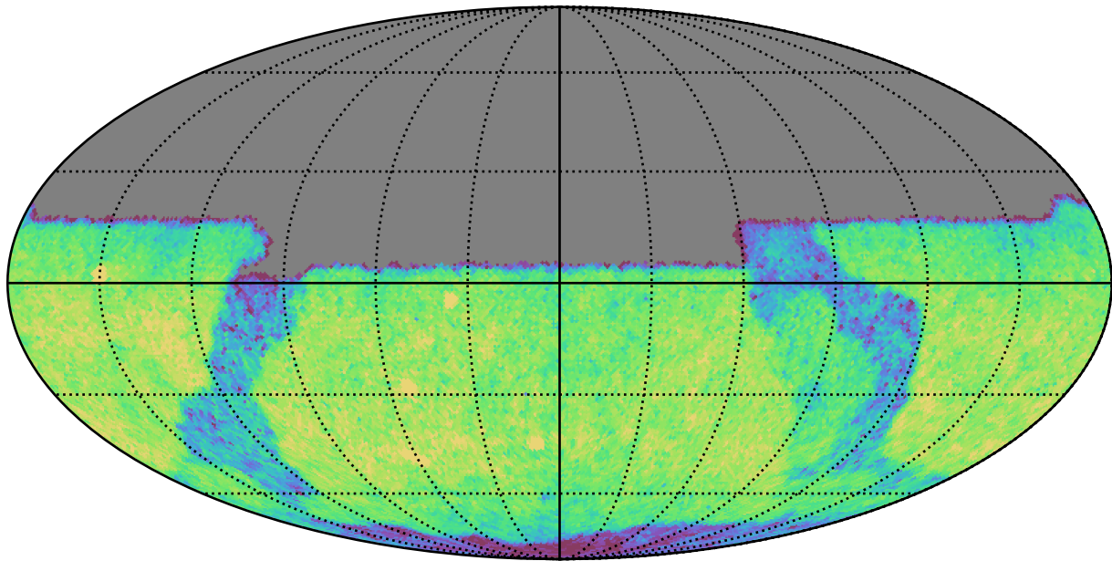
ddf_acor_sf25_lsf30_lsr50_v3.4_10yrs Yr 1 y band: CoaddM5
