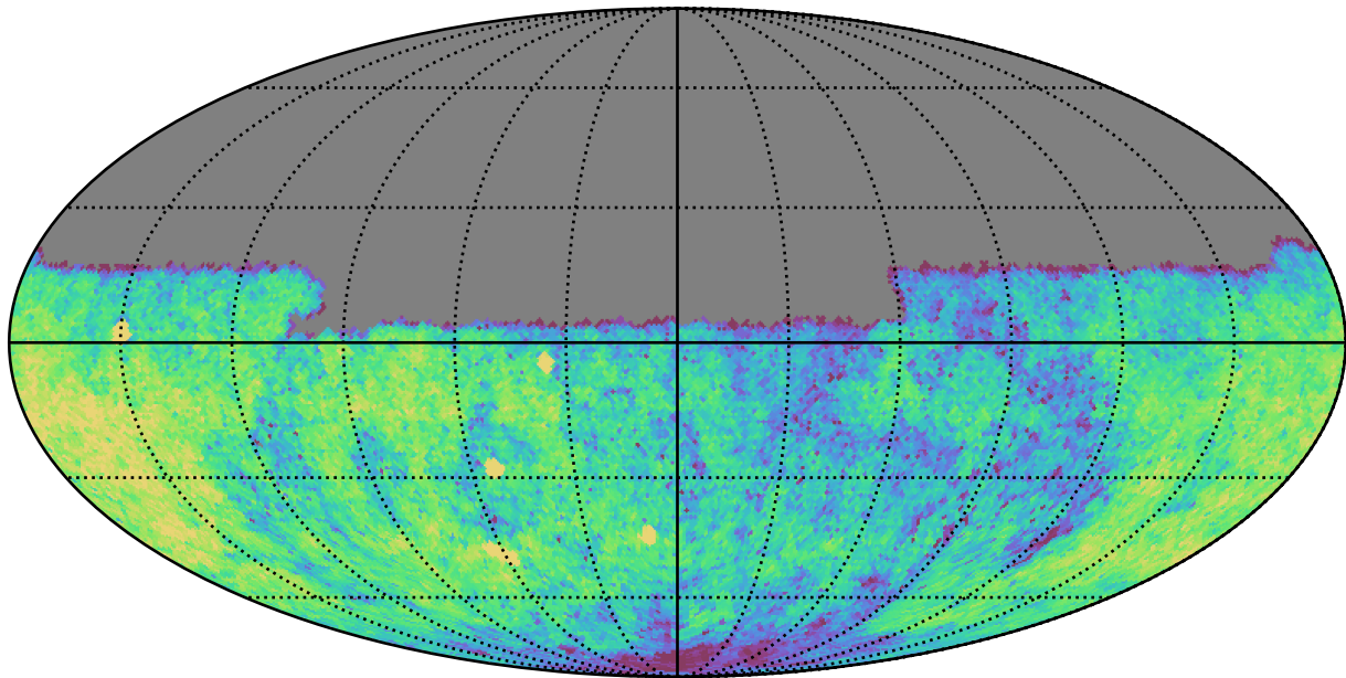
ddf_acor_sf25_lsf30_lsr50_v3.4_10yrs Yr 1 u band: CoaddM5
