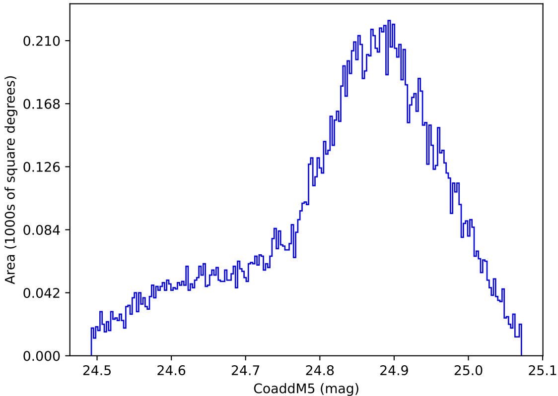
ddf_acor_sf25_lsf30_lsr50_v3.4_10yrs WFD y band: CoaddM5
